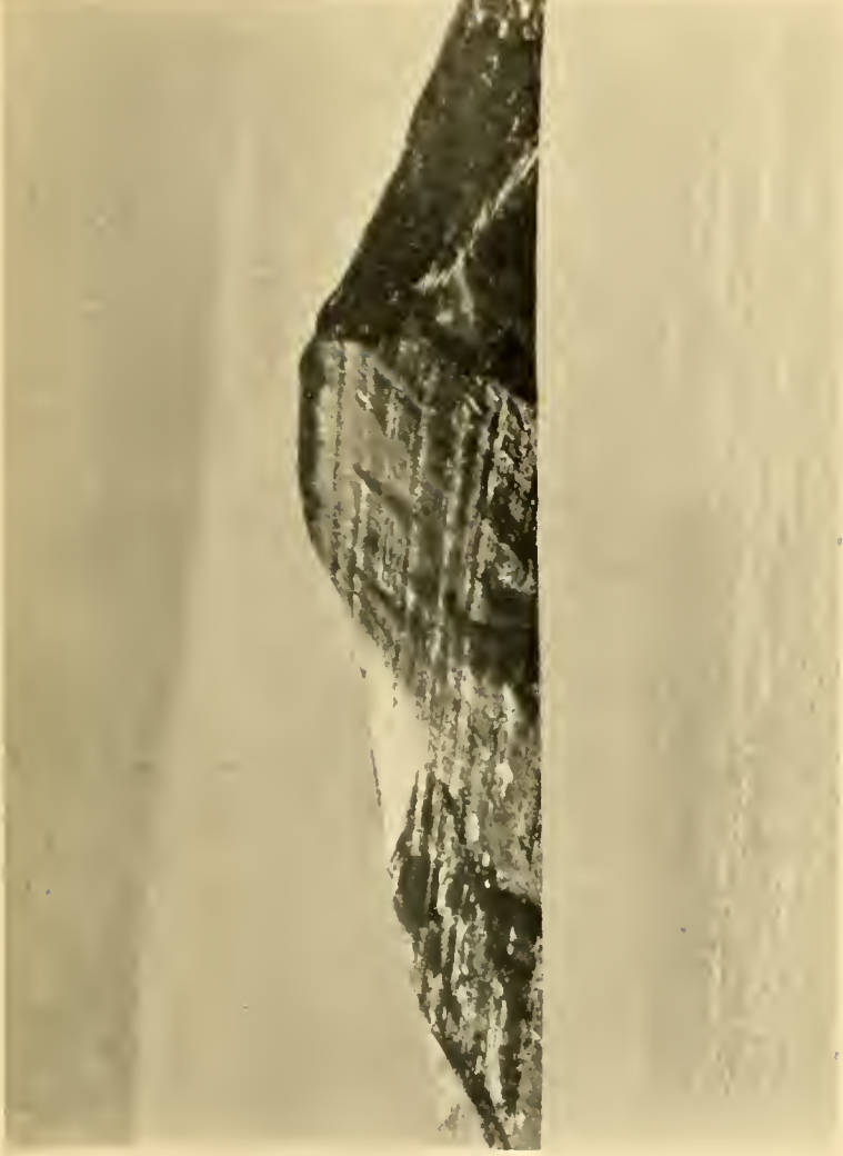
BUCKLEY ISLAND WHERE THE FOSSILS WERE FOUND
